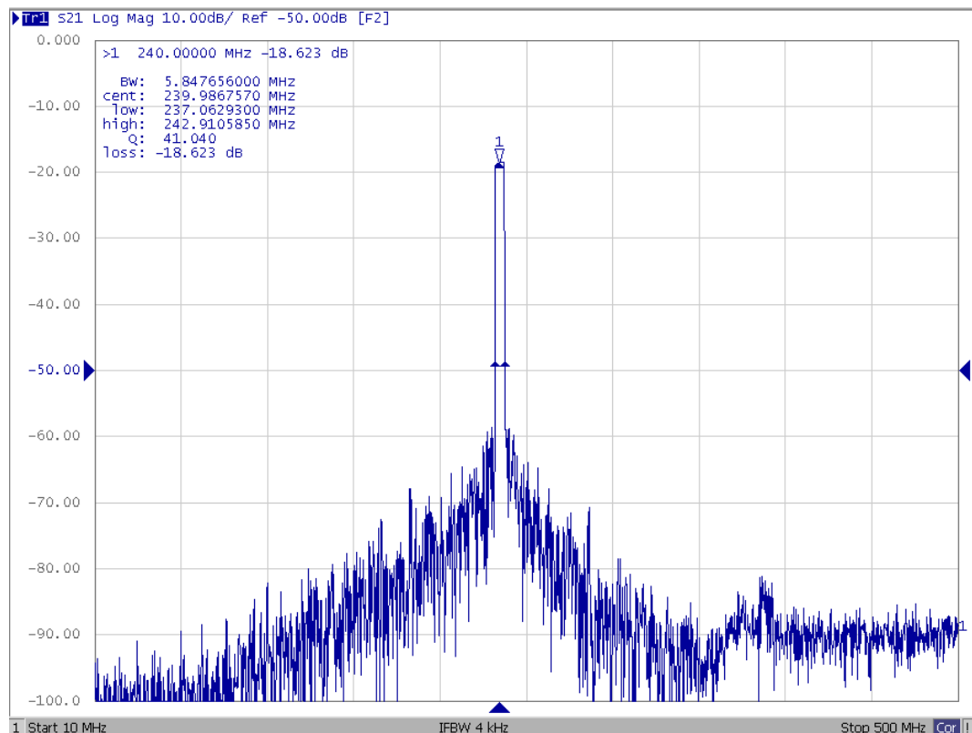
Fig4. Horizontal: 50MHz/Div Vertical: 10dB/Div
