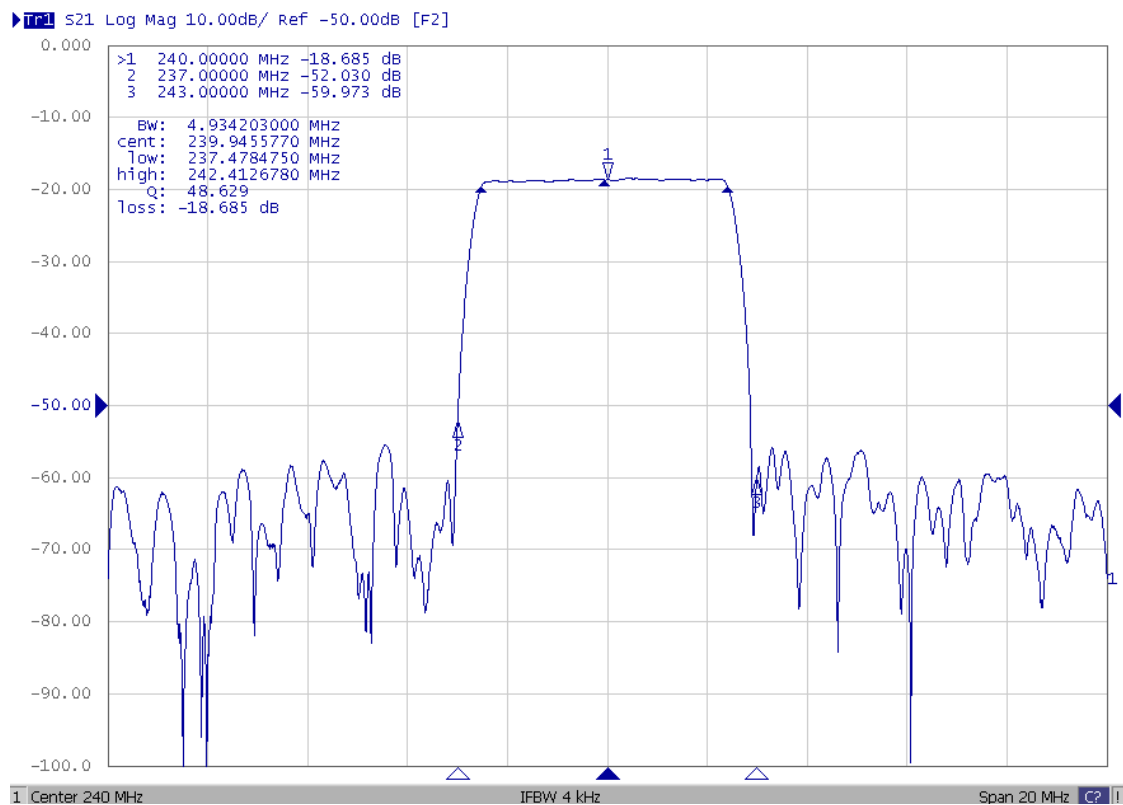
Fig1. Horizontal: 2MHz/Div Vertical: 10dB/Div
